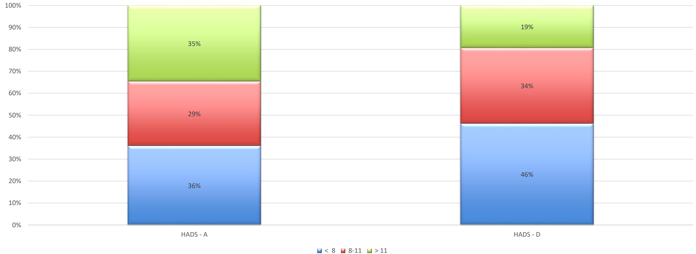
HADS Scores
